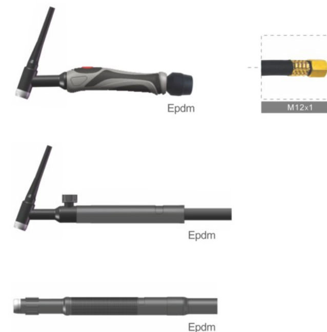
Complete torch-EURO
